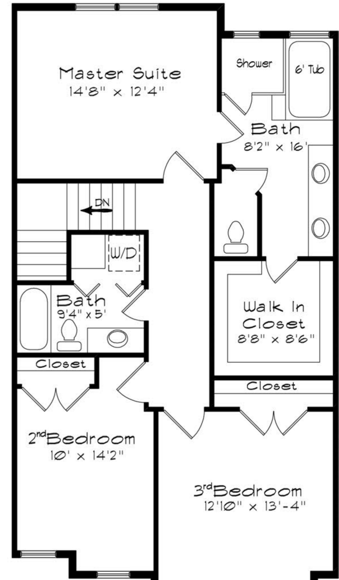
Upper Level
