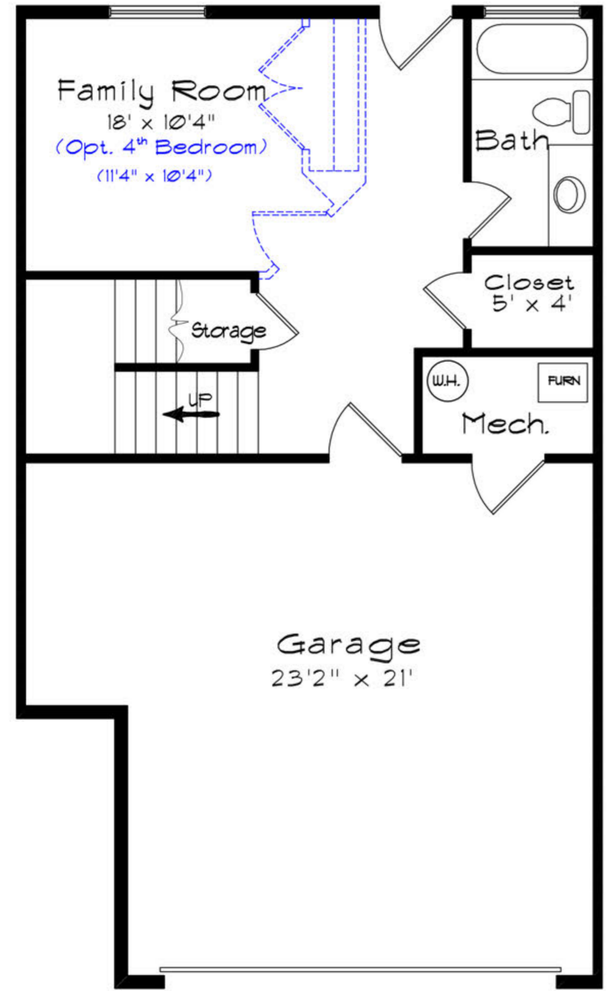
Garage Level
