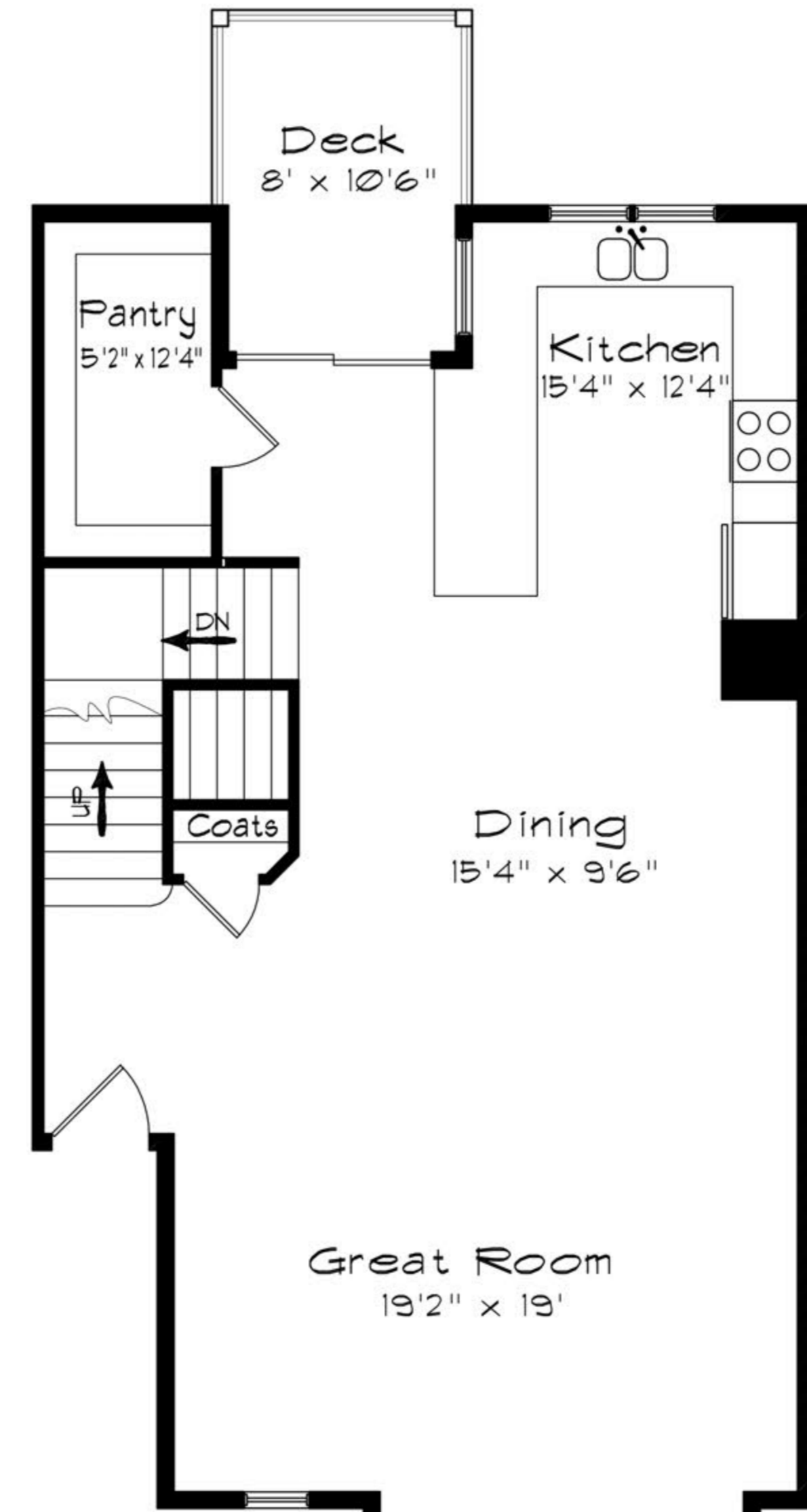
Main Level
